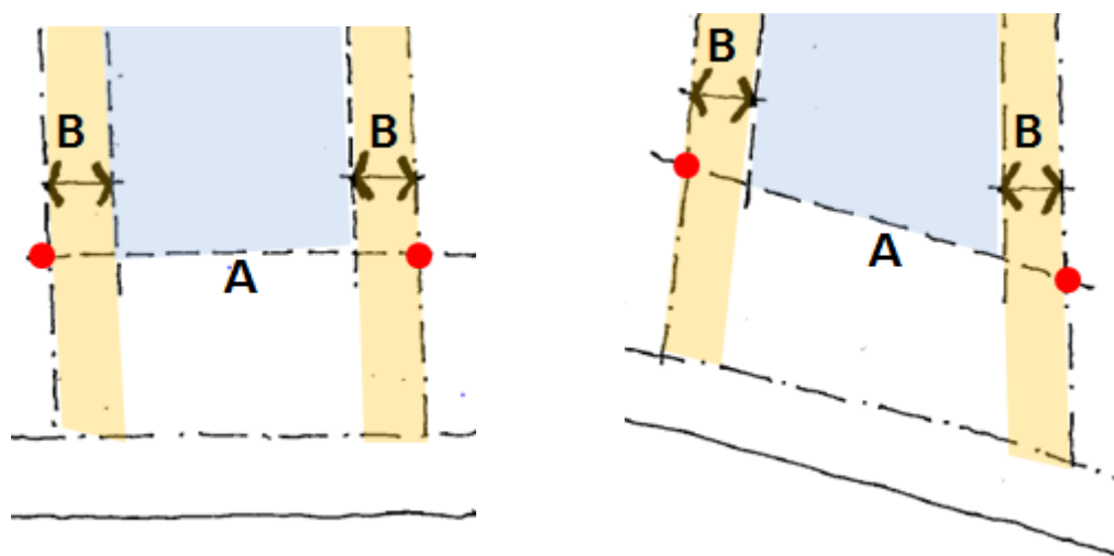
FIGURE 4 Side setback measurement, B depends on A
