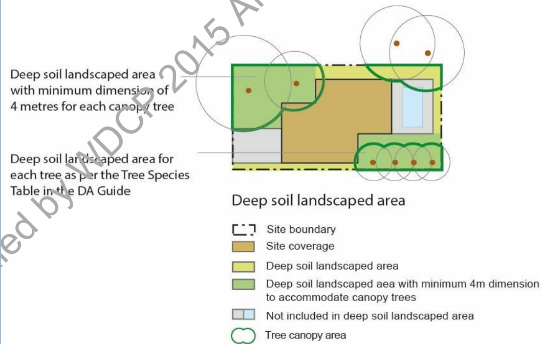
Figure 21 Calculation of deep soil landscaped area
